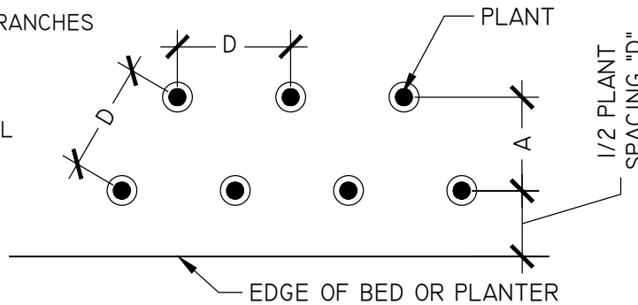
TRIANGULAR SPACING PLAN & CHART
