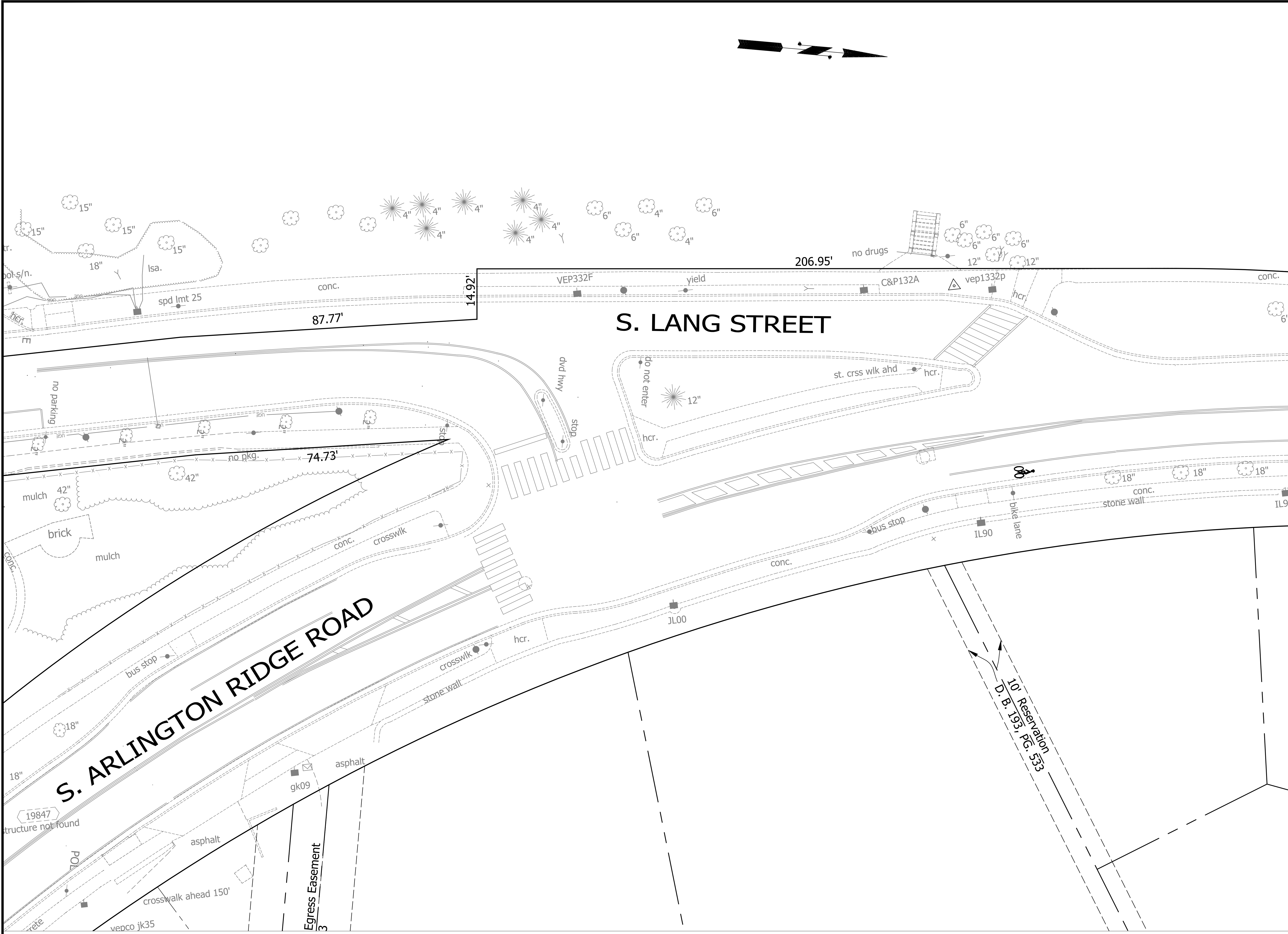
S ARLINGTON RIDGE RD AND S LANG ST INTERSECTION IMPROVEMENTS
