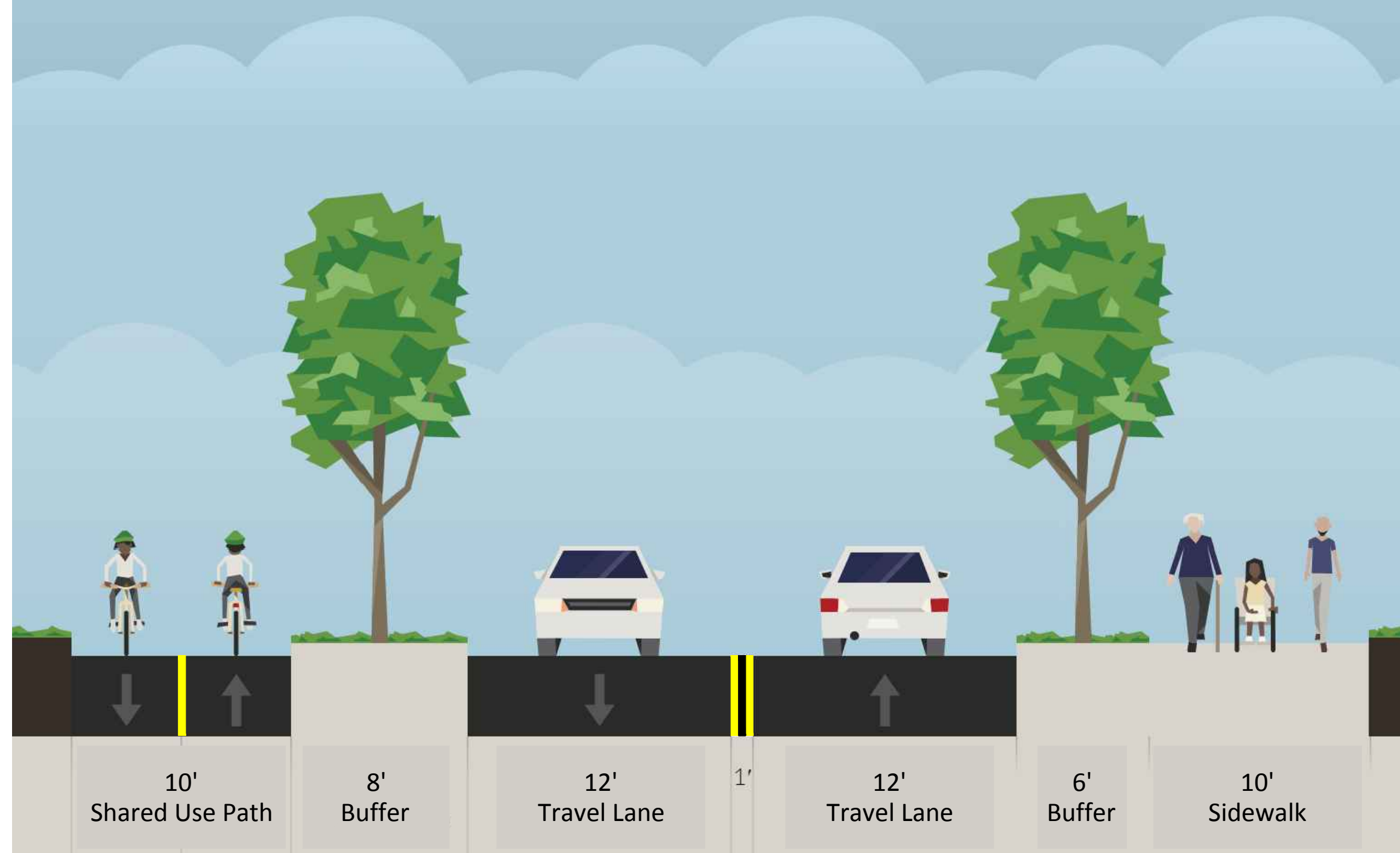
Typical Section View
